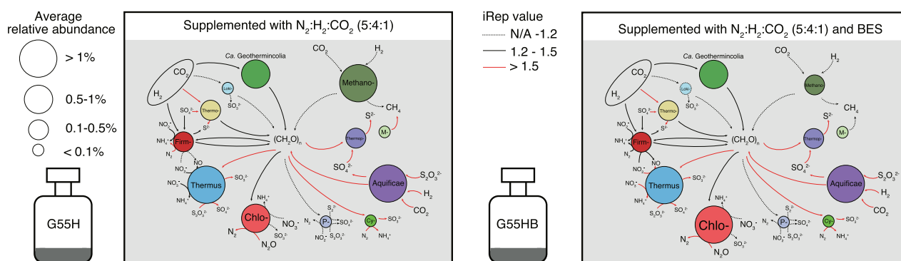
Fig. 7 Genome-resolved metabolic models in G55H and G55HB treatments. The metabolic models are based on the 105 representative MAGs. Methano- Methanobacteria , M- Methanomethylia , Loki- Lokiarchaeia , Desulf- Desulfurococcales , Thermo-
